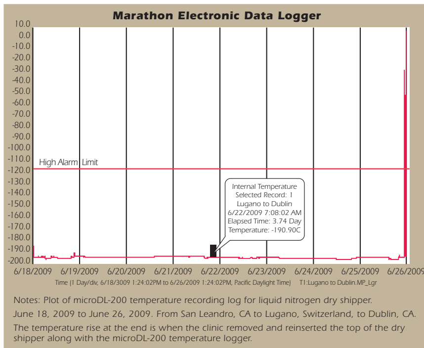
An example plot of temperature data for an 8 day international shipment.
